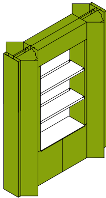
KIT VITRINA 2400 RW-KVIT-2400 1820x654x2400 mm.
